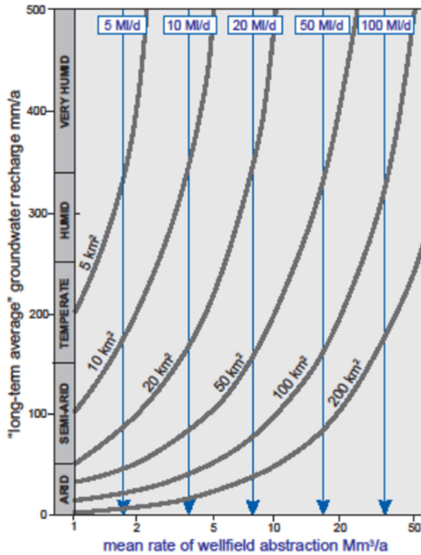
Figure A5 Variation in land area needed for complete protection of a groundwater or wellfield source.
