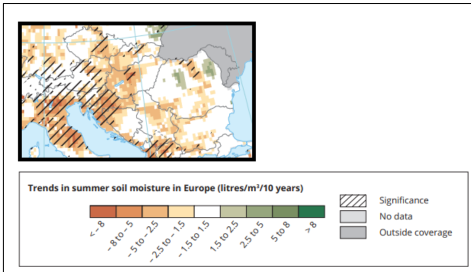
Figure 4: Trends in summer soil moisture
