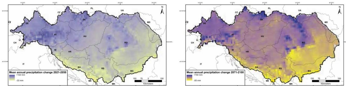
Figure 6: Estimated annual mean precipitation trends in the Danube region 2021–2050 and 2071-2100
