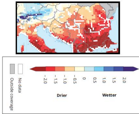
Figure 7: Changes are presented as mean multi-model change between 1961-1990 and 2021-2050 using 12 Regional Climate Models (RCMs); with red indicating drier and blue indicating wetter conditions.
