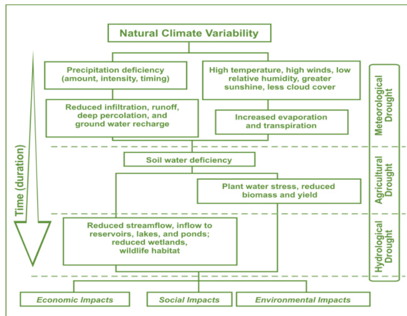
Figure 1: Sequence of drought occurrence and impacts for commonly accepted drought types. All droughts originate from a deficiency of precipitation or meteorological drought but other types of drought and impacts cascade from this deficiency.
