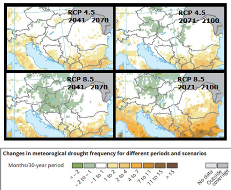
Figure 5: Changes in meteorological drought frequency for different periods and scenarios. Drought frequency is defined in this case as the number of months in a 30 year period with the Standardised Precipitation Index accumulated over a 6 month period (SPI-6) having a value below -2
