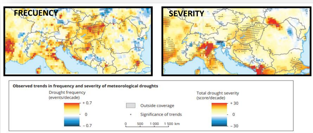
Figure 3: Trends in frequency and severity of meteorological droughts between 1950 and 2012. Trends are based on a combination of three different drought indices - SPI, SPEI and RDI accumulated over 12-month periods. Dots: trends significant at \geq 95\% .
